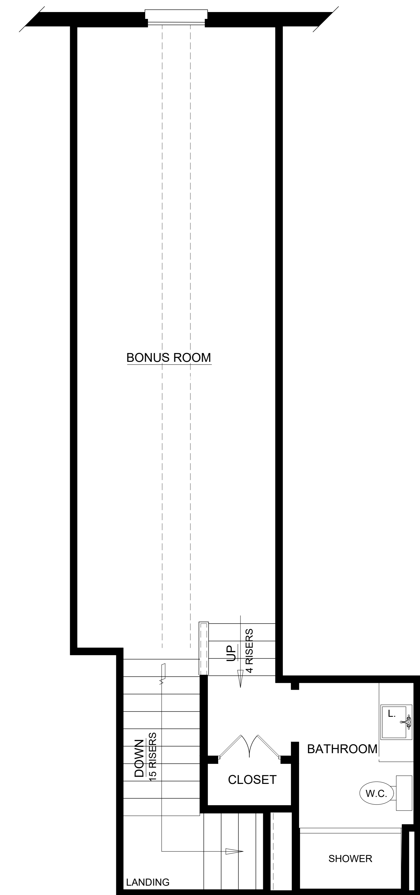
SECOND LEVEL FLOOR PLAN
