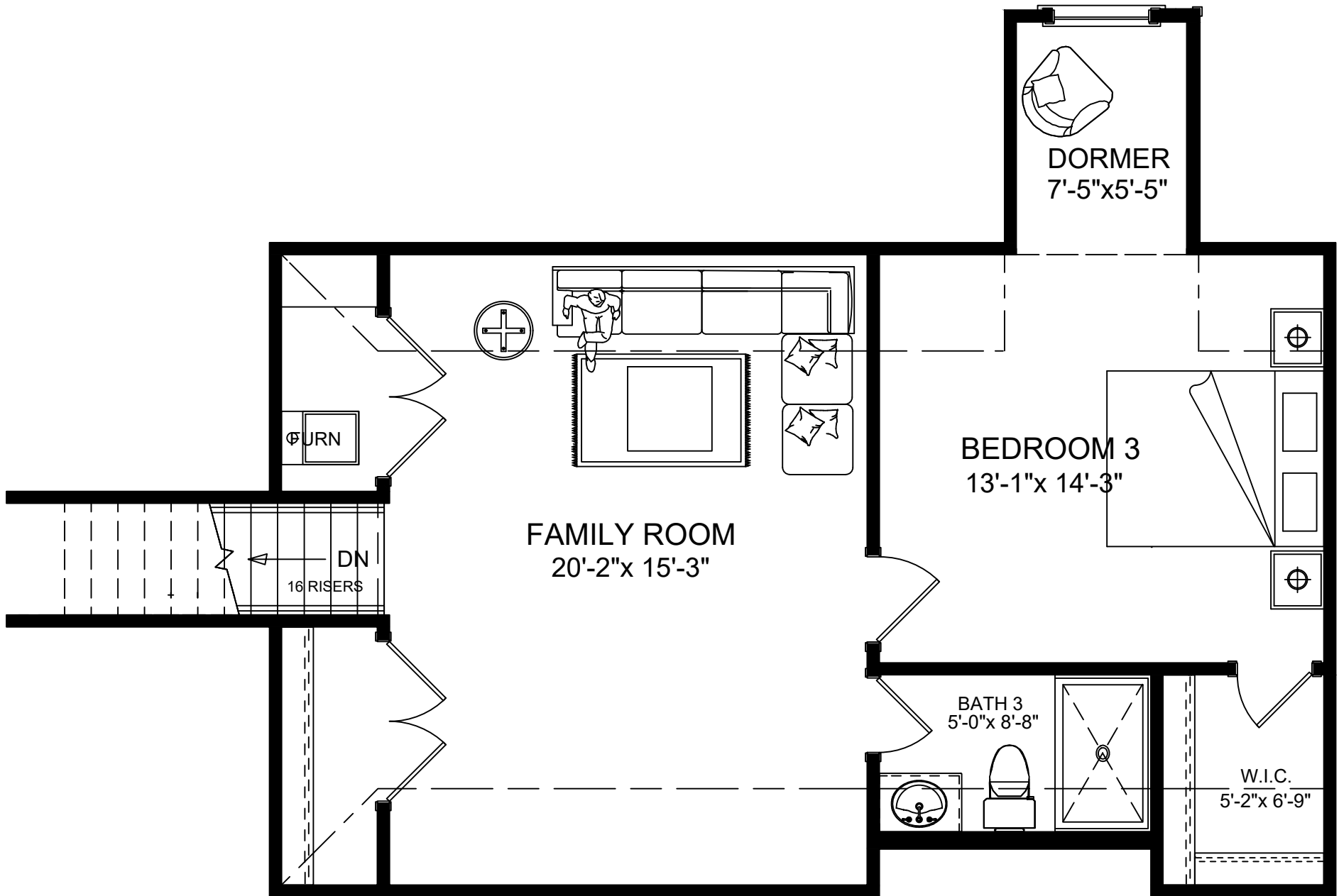
2nd FLOOR
